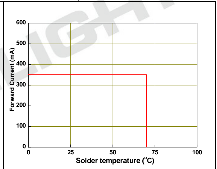
Forward Current Derating Curve, Derating based on T_{j\text{MAX}}=125 at torch mode
